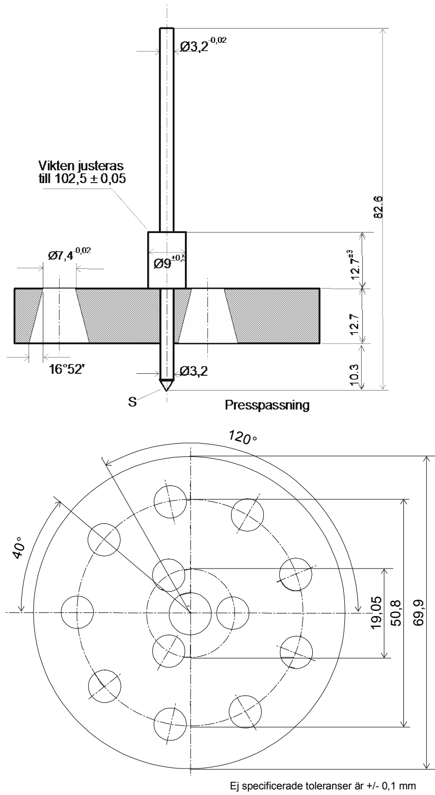
Figur 1: Penetrometer
